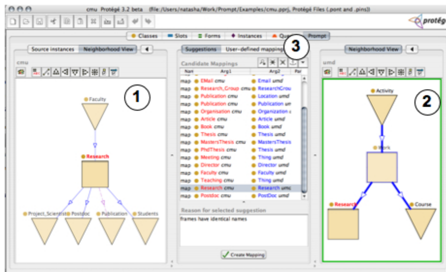
Fig. 5: PROMPT's mapping component with the interface plugin. Area (1) and (2) show the neighborhood's of the source and target terms of the currently selected suggestion. Area (3) shows the location of the filter button. The neighborhood display makes it clear that the two classes have different meaning in the two ontologies even though their names are the same ( Research ).
