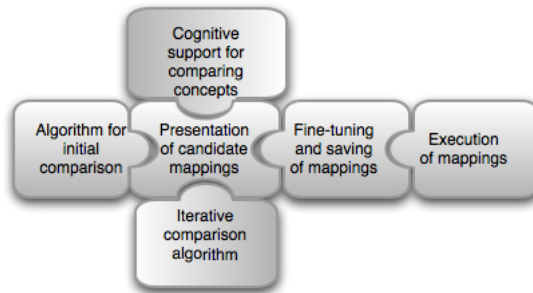
Fig. 3: Configurable steps in the PROMPT plugin framework. Developers can replace any of the components in the figure with their own implementation.
