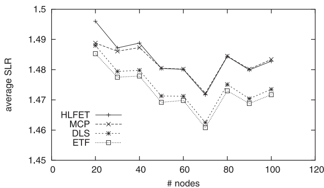
Fig. 6: Average SLR
