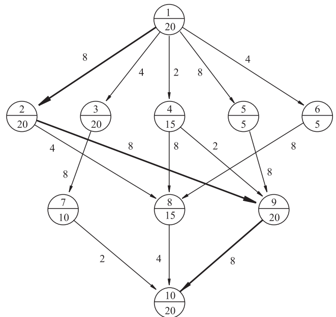
Fig. 1: Application directed acyclic graph (DAG)
