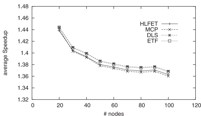
Fig. 7: Average Speedup
